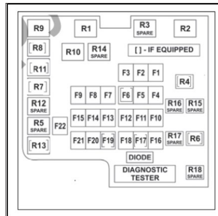
Cabin compartment fuse box layout
